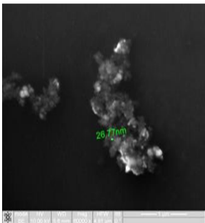
Fig.1. Study of magnetite nanoparticles with use microscope ion-electronic raster-type Quanta 200 3 D
